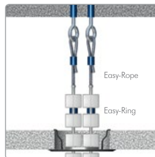
Mounting 2x KS Cube on raw-ceiling
